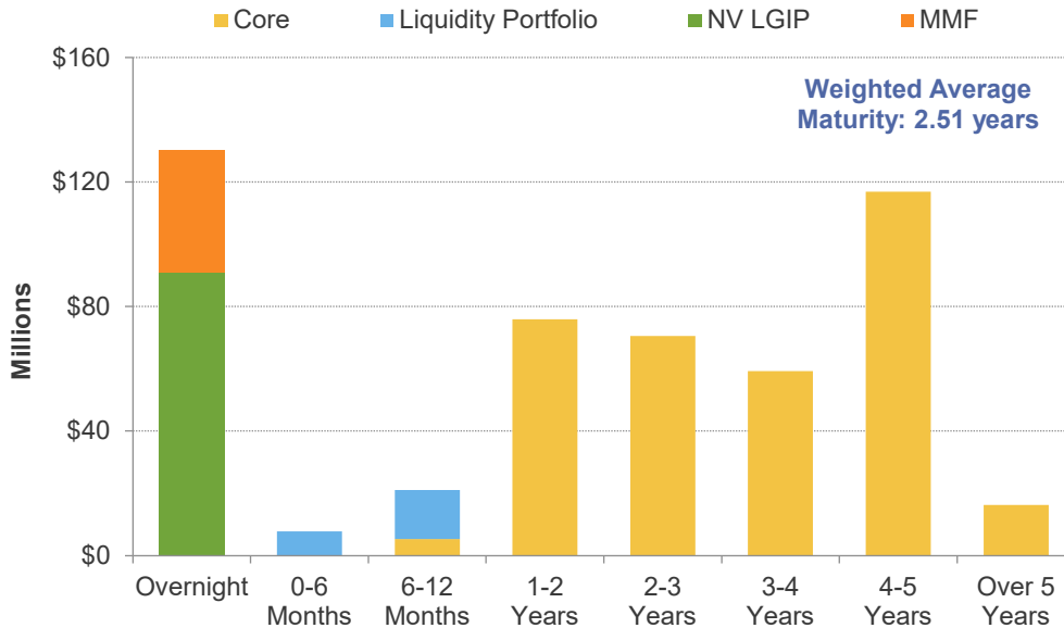
Maturity Distribution
