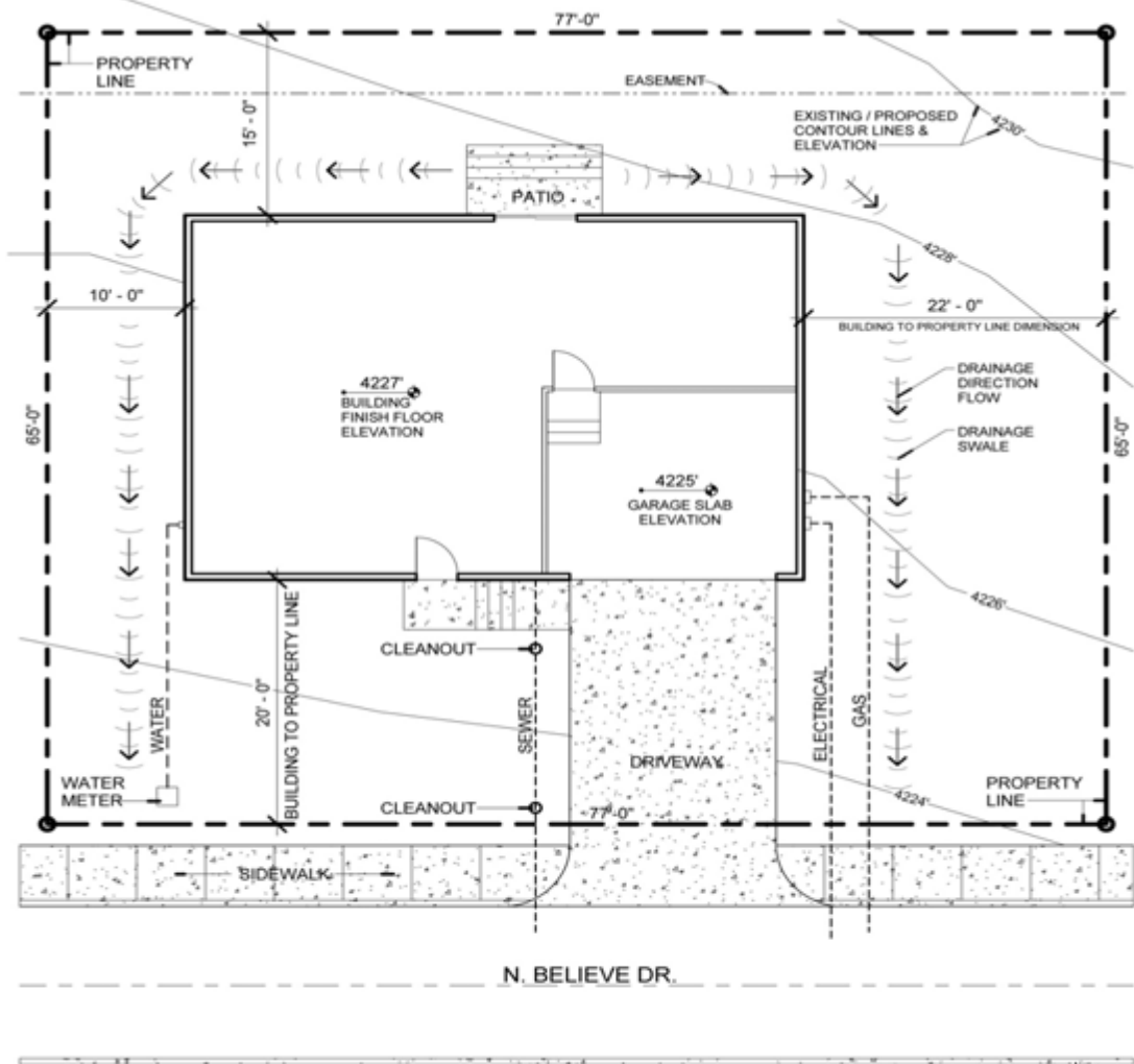
SAMPLE SITE PLAN
