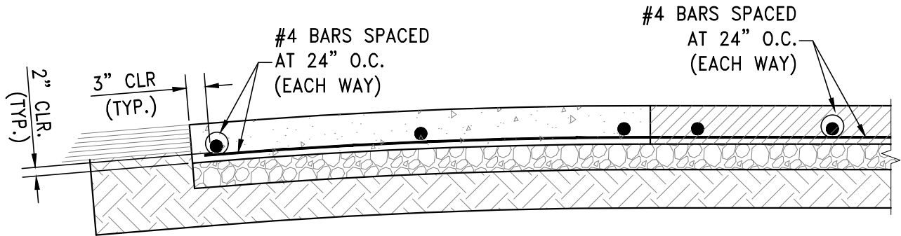
DETAIL A
