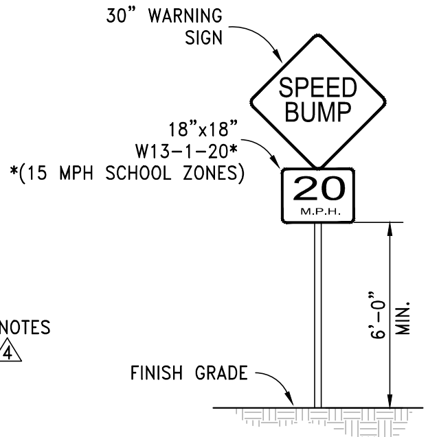
SIGN DETAIL 1
