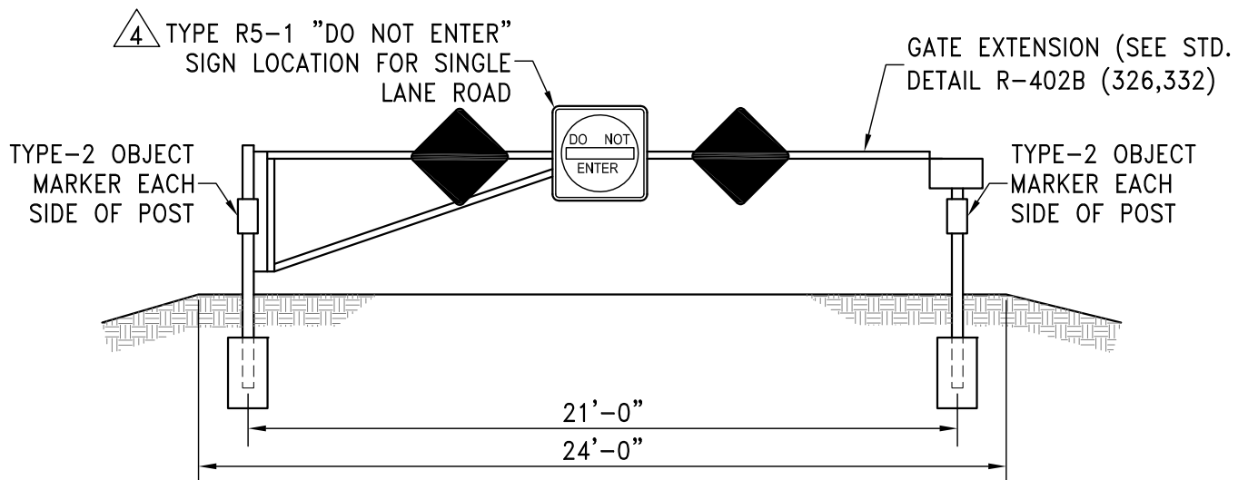
ELEVATION VIEW
